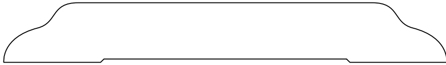
SAD5 5/8" x 4-5/8"
