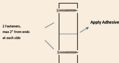
Butt Joint
