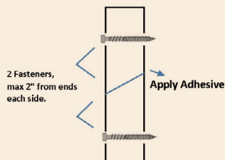
Scarf/Miter Joint
