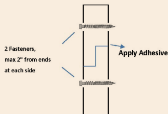
Shiplap Joint
