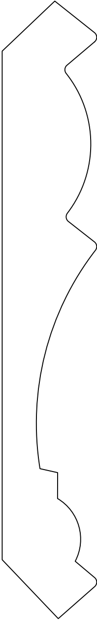
DCR612PP 1" x 6-1/2"
