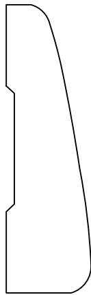
C106 11/16" x 2-1/4"
